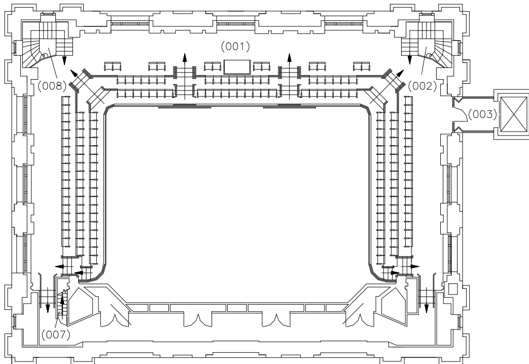
Lowell Hall Main Floor (Fixed Seating:190, Wheel Chair 4) And Balcony (Fixed Seating 162, Wheel Chair 4)
